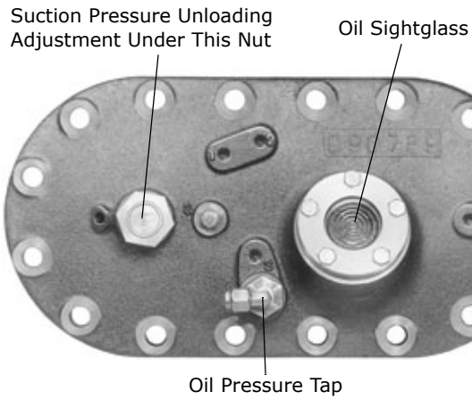
Figure 52. Suction Unloading Handhole Cover
