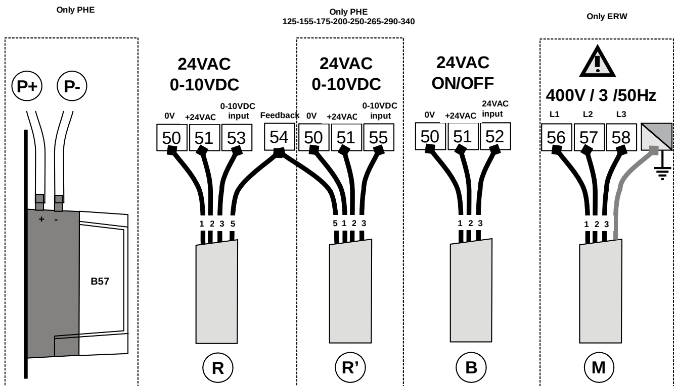
Figure 8 - Connections
