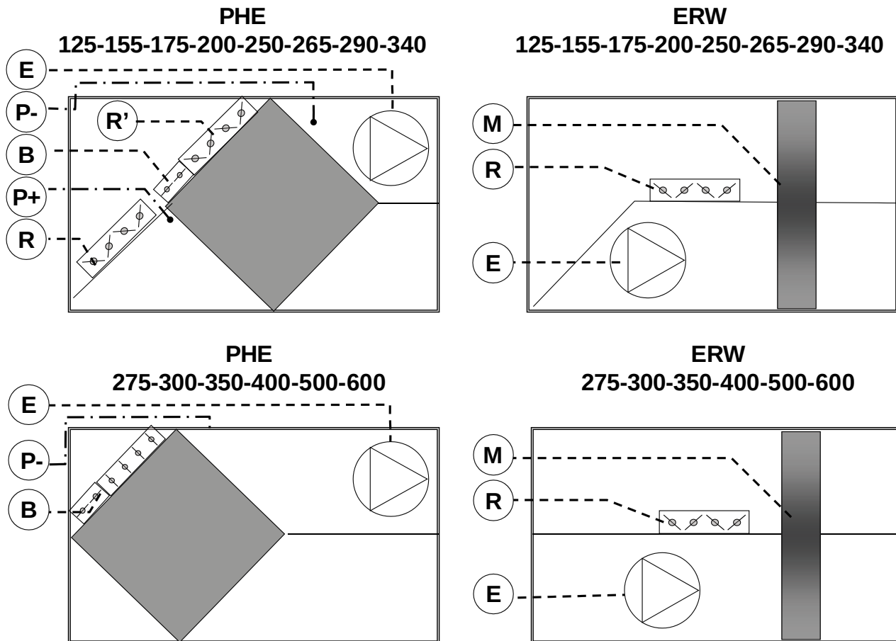
Figure 6 - Connections
